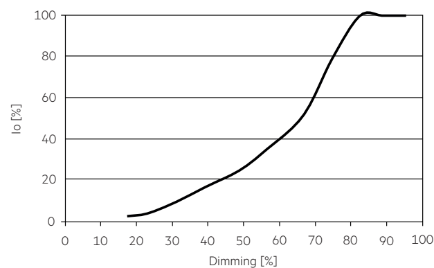
Output current vs dimming
